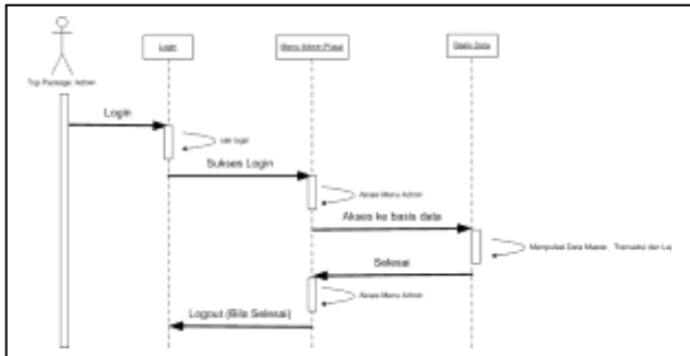
Sequence Diagram Admin Pusat
