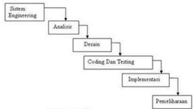
Model Waterfall
