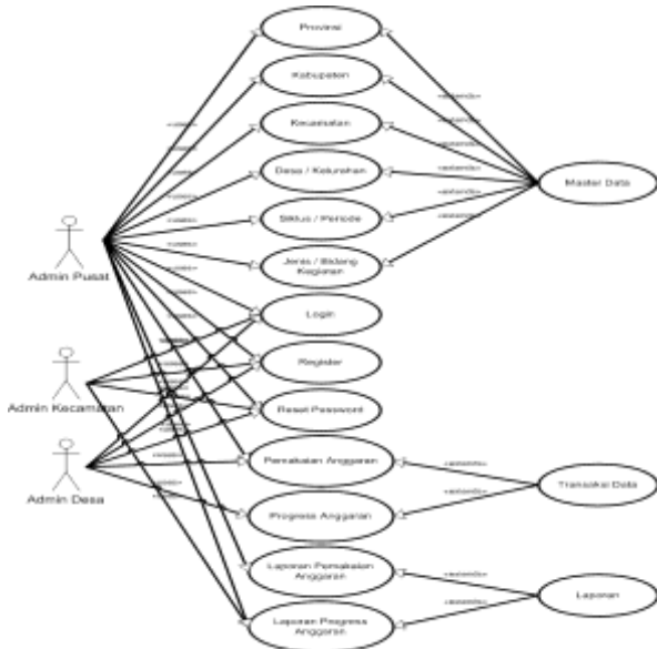
Use Case Diagram System Usulan
