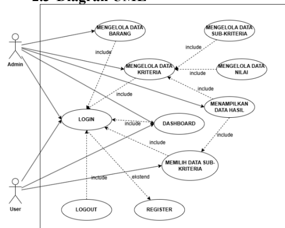
Gambar 1. Use Case Diagram Sistem
