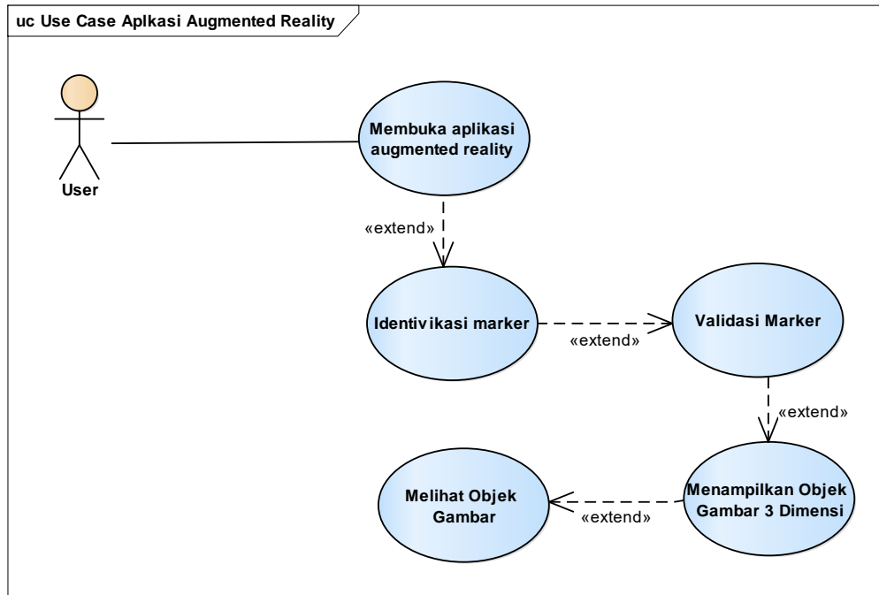
Gambar 3. 1 Usecase Diagram
