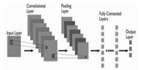
Figure 1. Convolution Neural Networks (CNN) architecture
