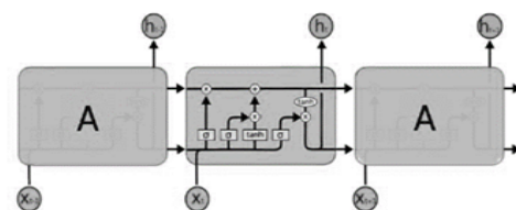
Figure 2. LSTM Architecture
