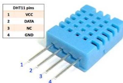
Gambar 5. Sensor DHT11
