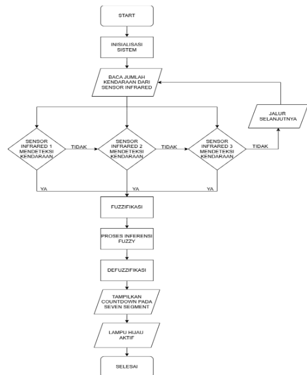
Gambar 5 Flowchart Sistem
