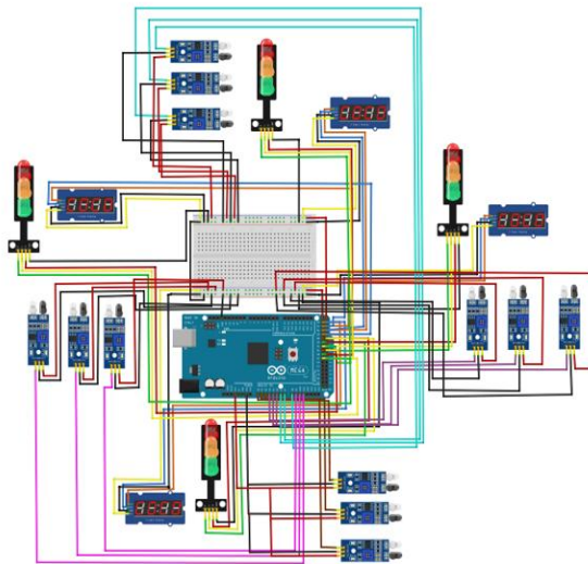
Gambar 4 Rancangan Hardware
